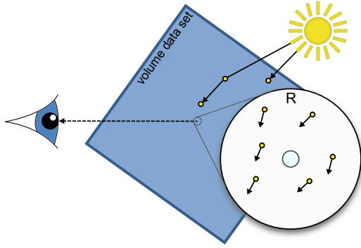
Figure 17: Photon mapping sends light particles into the scene and then collects all photons within a radius R to approximate the in-scattered radiance.
