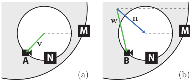
Figure 5: When the camera reattaches to a node, its coordinate system changes. While the old location A is expressed relative to N as \mathbf{v} , the new location B is expressed relative to M as \mathbf{w} - \mathbf{n} instead.
