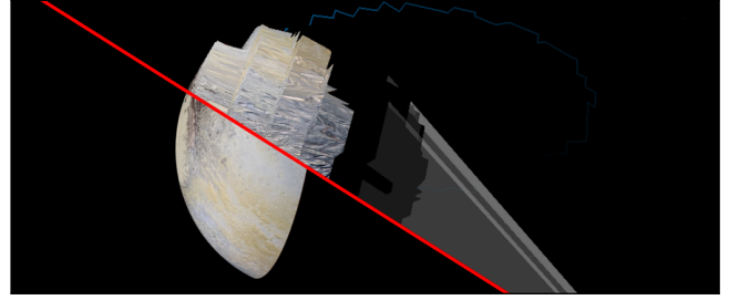
Figure 3: Floating point error at Pluto. Floating point quantization are visible at Pluto's distance of 5.1 billion km from the Sun using PSC. Our method achieves high fidelity renderings while still representing objects with single precision floating point numbers.
