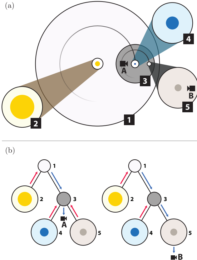
Figure 4: A potential scene graph consisting of two translation nodes for the solar system and the Earth system (1, 3) and three rendering nodes for the Sun (2), Earth (4), and the Moon (5). Cameras (A, B) can be attached to different nodes, thus avoiding the introduction of large, error-prone translation values. (a) shows the nodes relative location, whereas (b) shows their organization in a graph. The arrows represent local upwards (red) and downwards (blue) transformations.
