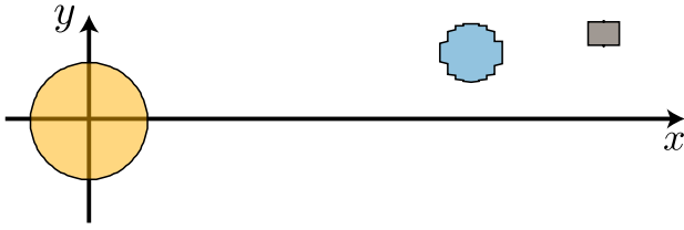
Figure 2: An illustration of the effects of limited coordinate precision where the number of mantissa bits is limited to 5 when visualizing a system analogous to a world coordinate system in a scene graph. Increasing distance leads to decreasing precision.
